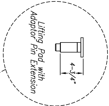
Adaptor Pin Extension
